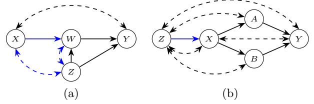
Figure 2: Edges shown in blue are those whose expansion identifies p(\mathbf{y}|\text{do}(\mathbf{x})) . Theorems 1, 1, and 1 fully resolve (a), but not (b).
